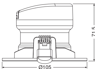
GIMBLE DL LED PERF 60X90MM 10W/830
